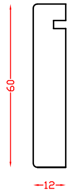
Cornice Design
